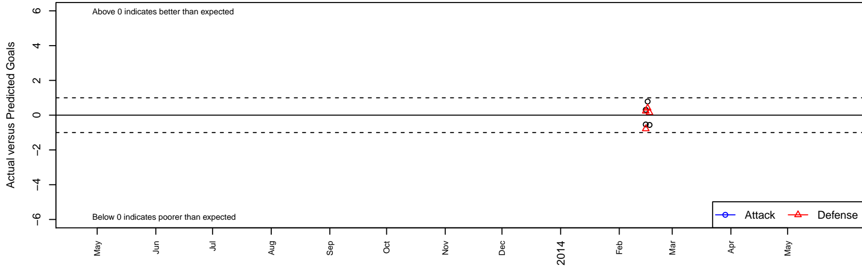
Arsenal Colorado Gold G01 Dots are actual minus expected GF (blue circles) and GA (red triangles). Blue line is smoothed change in attack strength. Red is smoothed change in defense strength.
